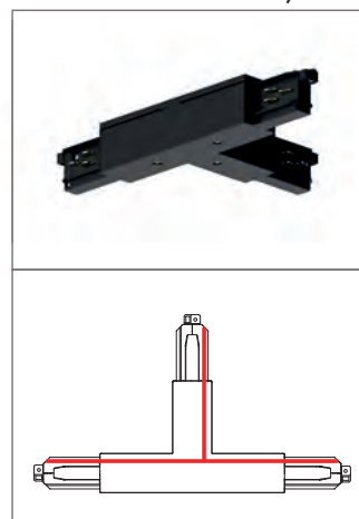
T - Feed /9016
