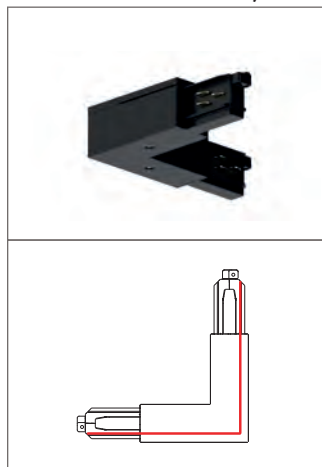
L - Feed /9012
