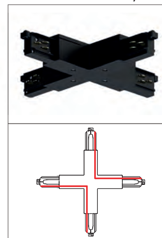
X - Feed /9017
