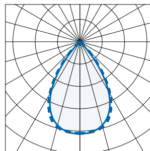
65° optic
