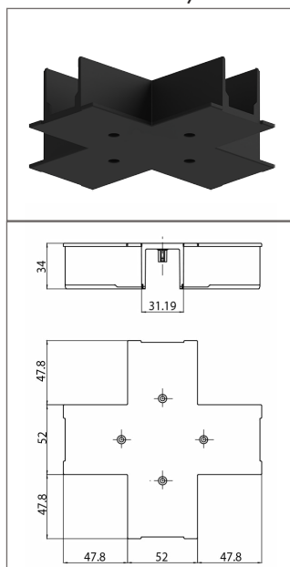
X - Feed Cover /S-9017-R
