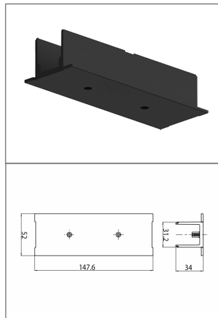
Middle Feed Cover /S-9010-R
