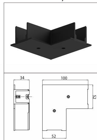
L - Feed Cover /S-9011-R
