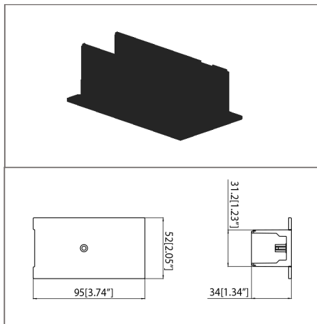
End Feed Cover /S-9001-R
