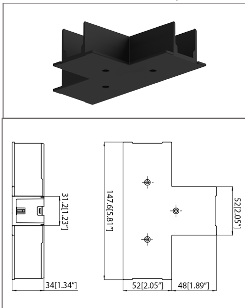
T - Feed Cover /S-9013-R
