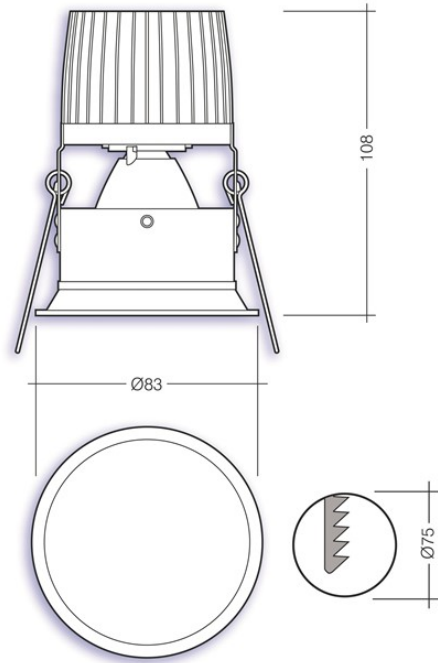
40° reflector
