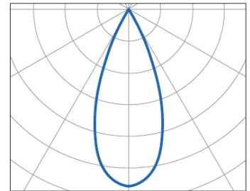
40° reflector
