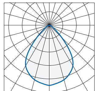
Wide 90°
